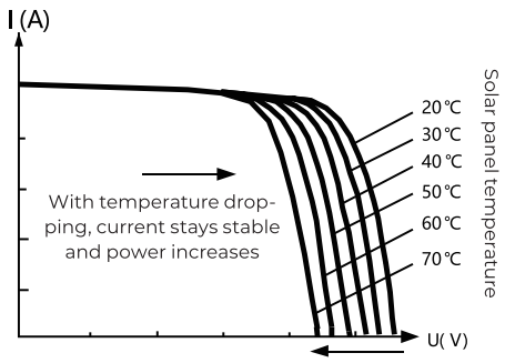
Open-circuit voltage decreases with rising temperature
