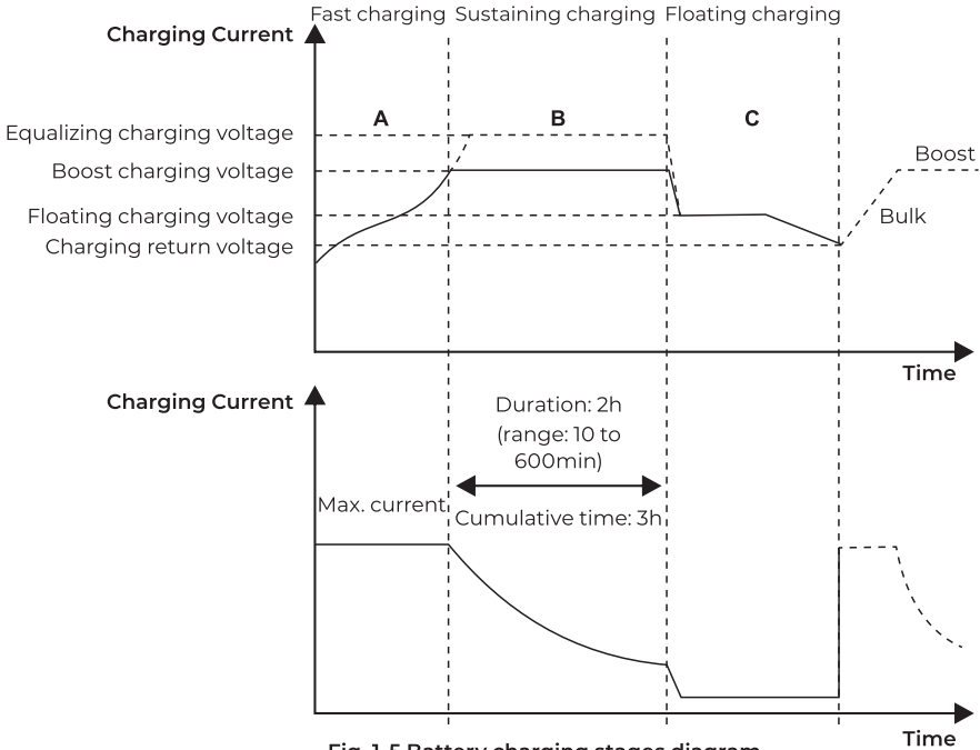
Fig. 1-5 Battery charging stages diagram
