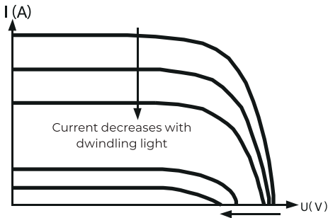
Open-circuit voltage decreases with dwindling light
