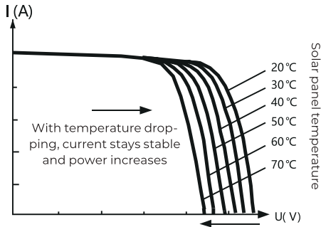
Open-circuit voltage decreases with rising temperature
